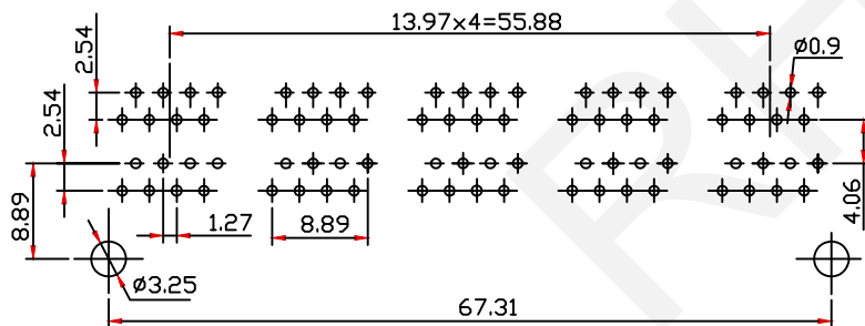
PCB Layout
